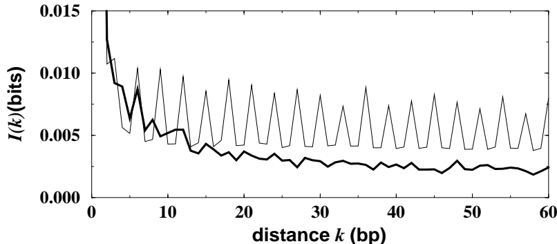
Figure 1: Mutual information function, I(k) , of coding DNA (thin line) and noncoding DNA (thick line) from the set of animal DNA in GenBank 111. We extract from files gbpri1.seq , gbpri2.seq , gbpri3.seq , gbrod.seq , gbmam.seq , gbvrt.seq , gbinv1.seq , and gbinv2.seq , all protein-coding exons and all introns with a minimum length of 300 bp, and we cut these sequences into non-overlapping fragments of length 300 bp, starting at the 5'-end. We compute the mutual information function of each fragment, and display the average over all mutual information functions (of exons and introns separately). While I(k) for noncoding DNA decays monotonically to zero as k increases, I(k) of coding DNA shows persistent period-3 oscillations.
