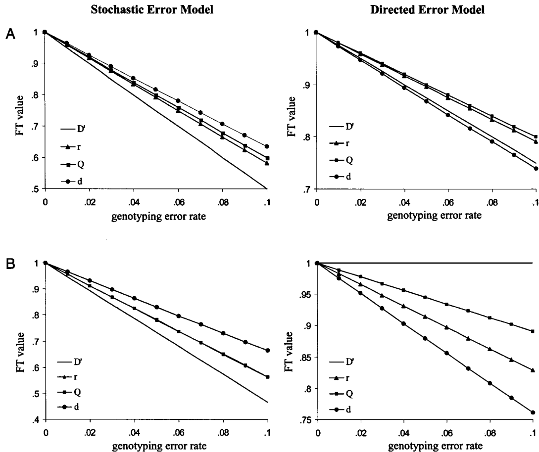
Figure 2 The effect that genotyping errors have on FT values, as a function of genotyping-error rate. In panel A, the haplotype frequencies are P_{AB} = .3 , P_{Ab} = .3 , P_{aB} = .1 , and P_{ab} = .3 ; in panel B, the haplotype frequencies are P_{AB} = .1 , P_{Ab} = .4 , P_{aB} = .3 , and P_{ab} = .2 . Note that, in panel B, the lines corresponding to r and Q for the SEM are nearly superimposable.
