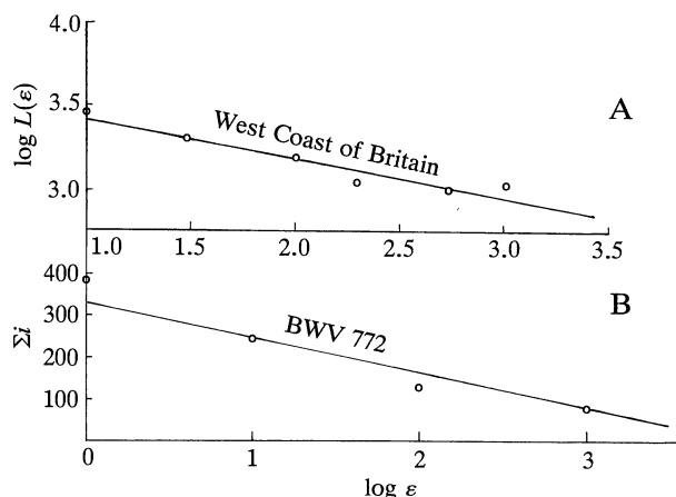
FIG. 1. Rate of decrease of coastline length L(\epsilon) (A) and decrease of music note intervals i (B) as a function of the “yardstick” length (see text for detailed explanation).
