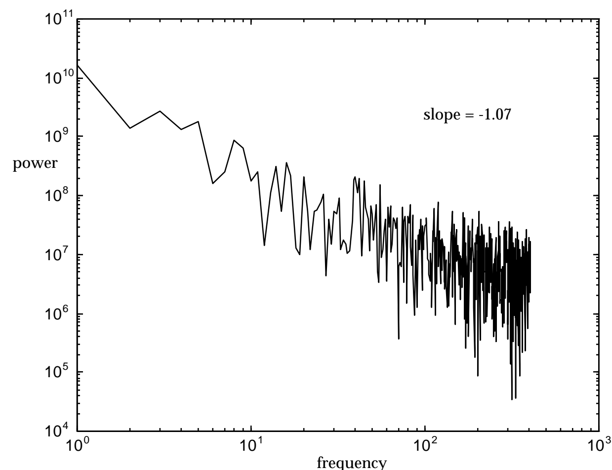
Figure 1: load force spectral power density for a single run
