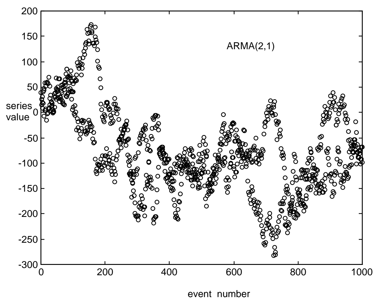
Figure 8: an ARMA-like time series from Eq (4) in a region of marginal stability, with \mathbf{a} = -\mathbf{b} = 1
