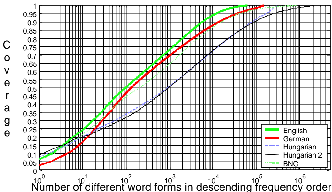
Figure 2. Corpora coverage by the most frequent words (logarithmic horizontal scale) of standard texts
