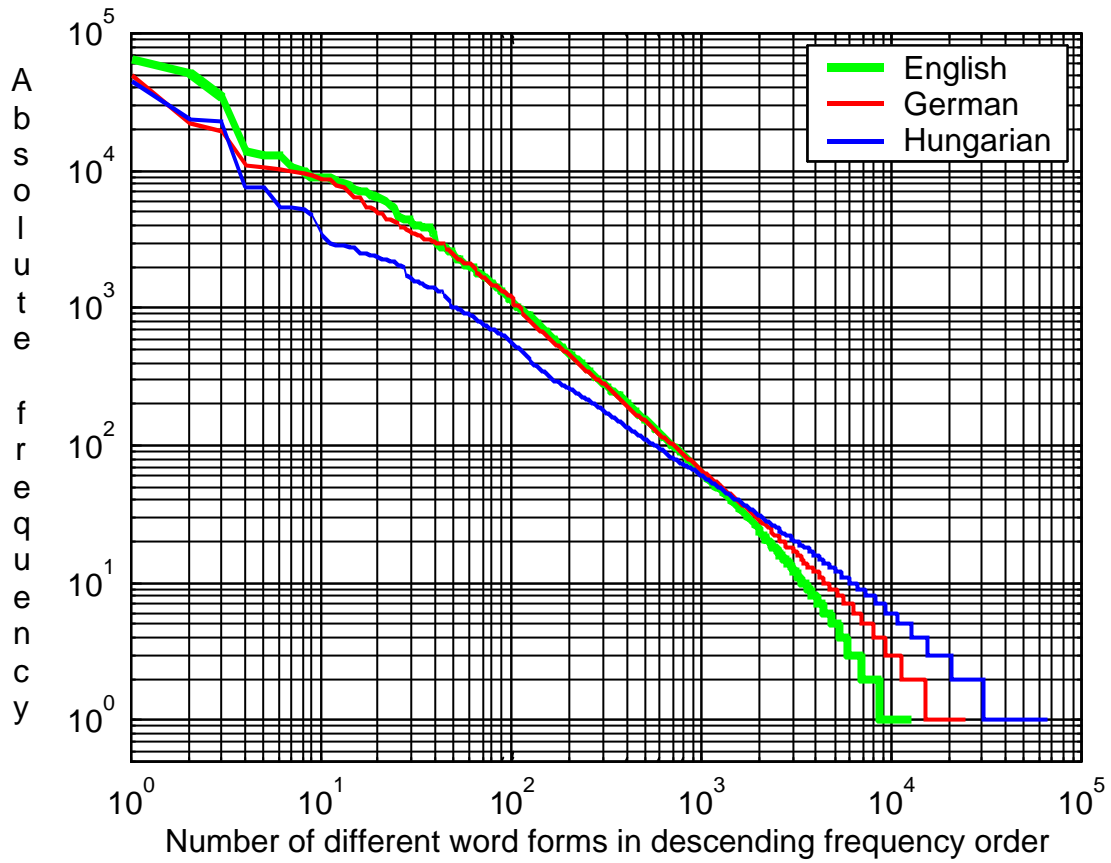
Figure 4. Ranking of Bibles
