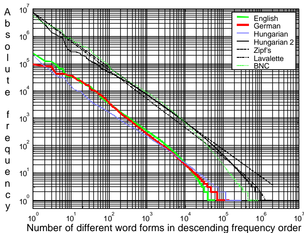
Figure 1. Ranking of standard texts
